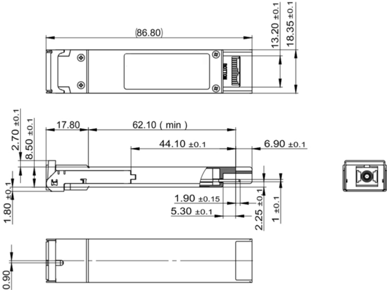
Figure 7 Package Outline
